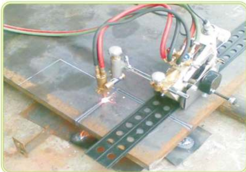
● Gas Cutting
